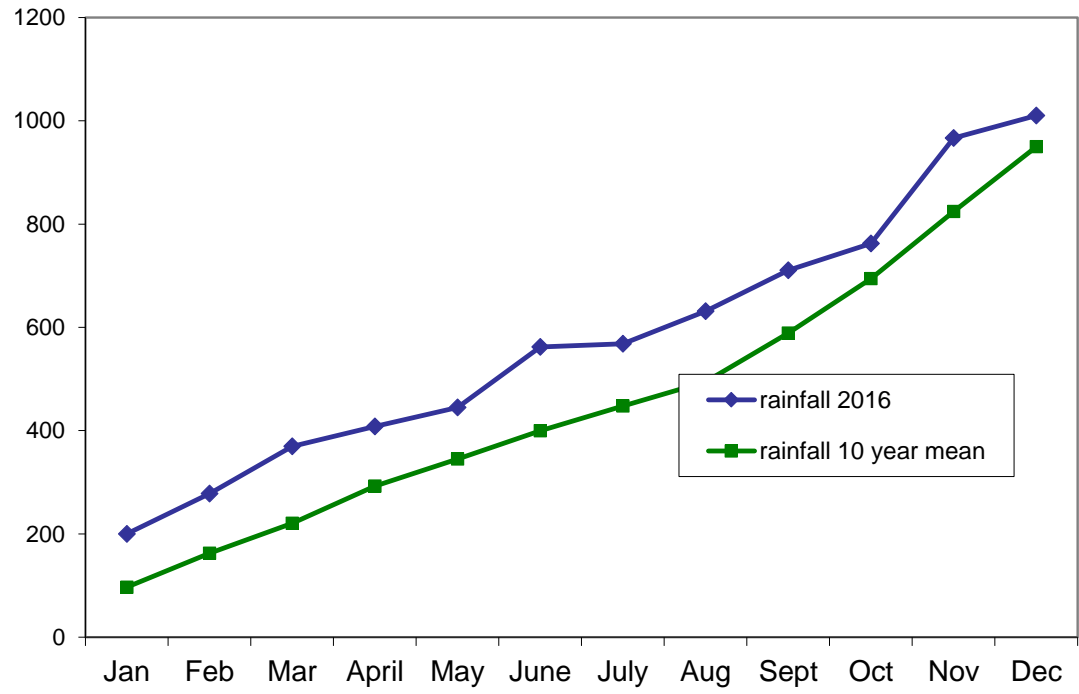
Cumulative Monthly Rainfall 2016 cf 10 year mean
